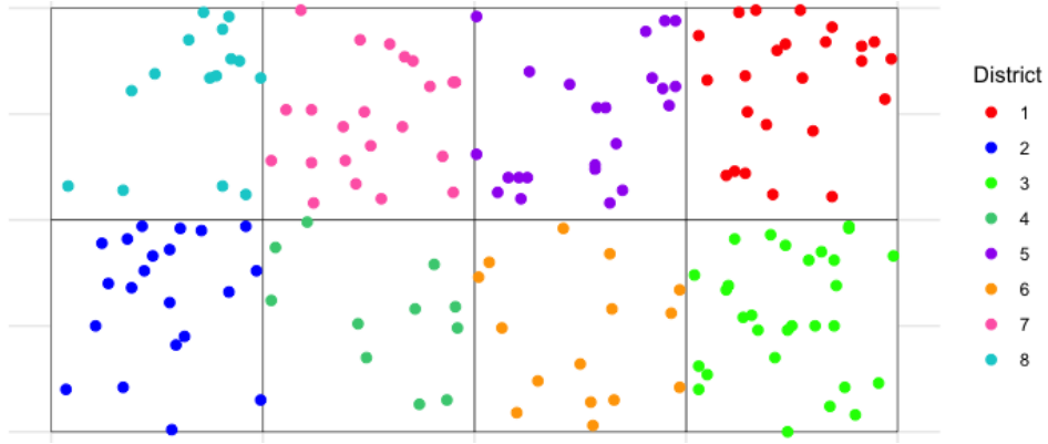
Figure 4: Example of simulated observation coordinates ( n=160 ) on a 2 \times 4 2 \times 4 grid of clusters
