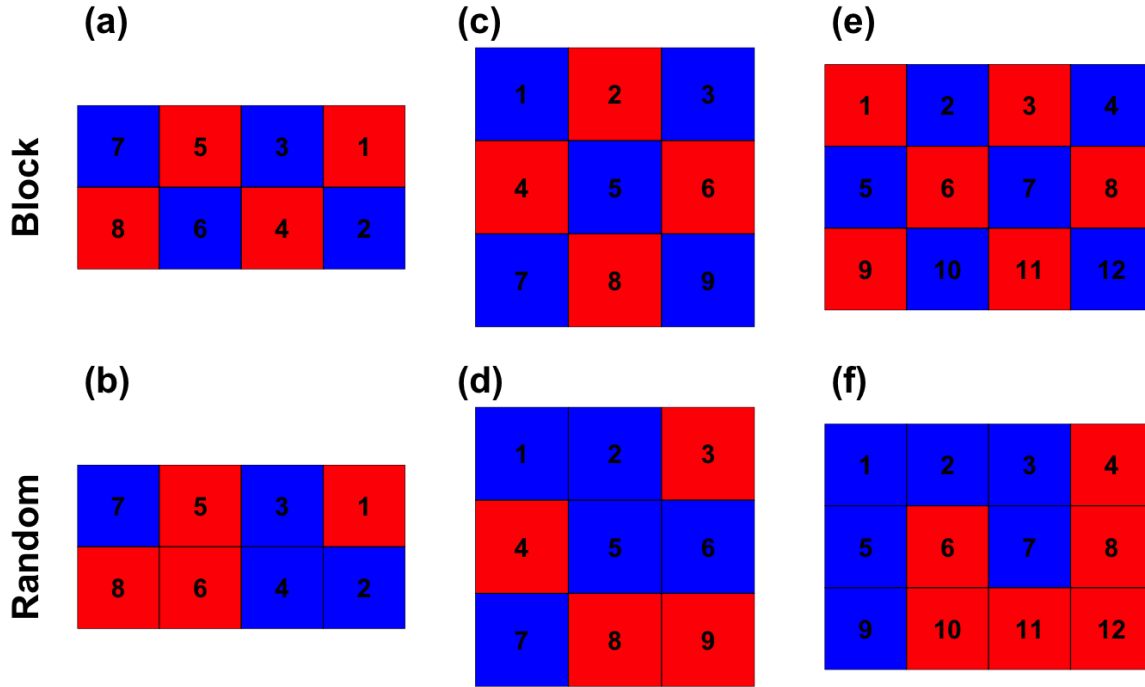
Figure 3: 2 \times 4 (left), 3 \times 3 (middle), and 3 \times 4 (right) spatial grids of intervention (red) and control (blue) clusters assigned via Block Stratified Sampling (top row) and Random Sampling (bottom row)
