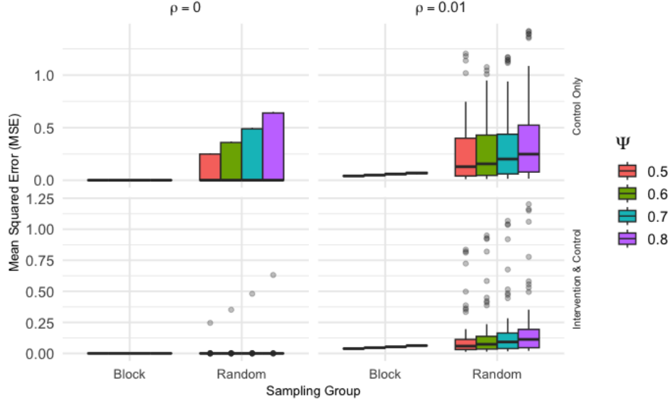
Figure 6: Intervention effect MSE for 3 \times 3 - 3 \times 3 cluster grid grouped by spillover effect magnitude, spatial dependence, sampling design, and spillover application type
